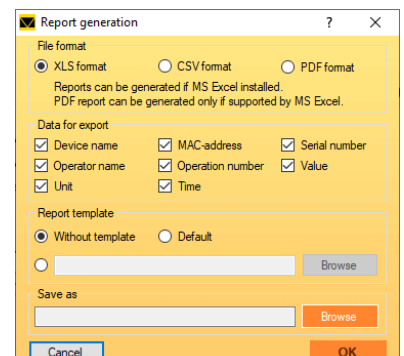
REPORT SAVING
