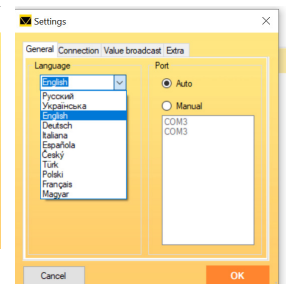
MULTILANGUAGE
